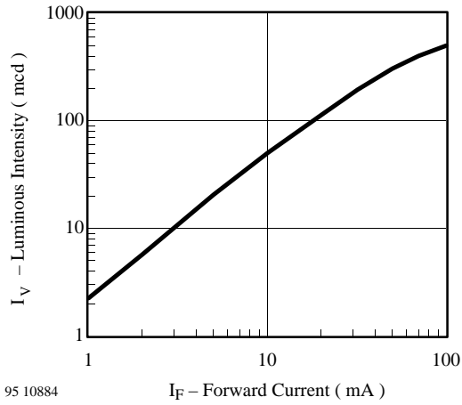
Figure 7. Luminous Intensity vs. Forward Current
